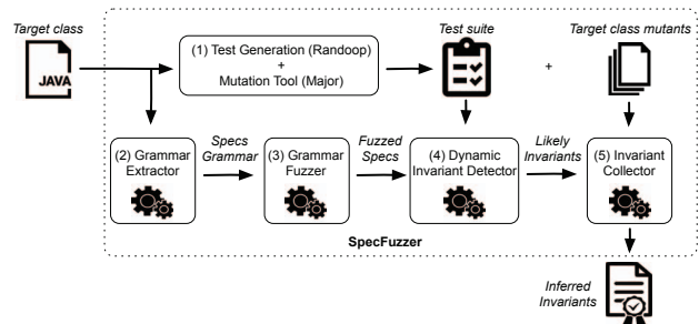
Figure 4: The SPECFUZZER workflow.
